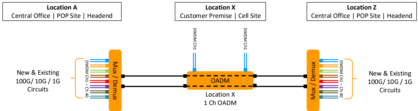
Figure 1: Linear OADM Diagram, 1Ch DWDM
