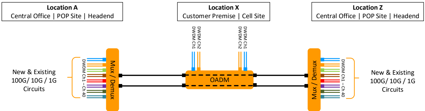
Figure 1: Linear OADM Diagram, 2Ch DWDM
