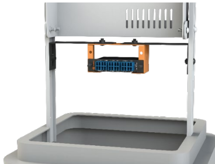
Figure 2: Pedestal bracket kit and magnet mount assembly. Shown installed in a two-post pedestal and equipped with a LGX module.
