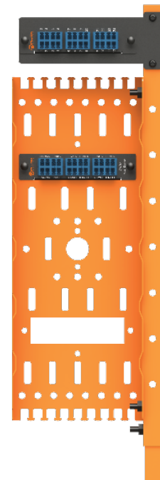
Figure 1: Plugin Optics 1 Slot LGX Bracket installed on a pedestal stake, with an LGX module inserted, directly above a universal mounting plate.
