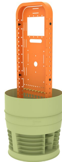
Pedestal kit: PLO-B-PED-1014 10-Inch Pedestal High Density Backboard Kit.
