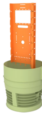
Pedestal Kit: PLO-TLP-TPED-SGP0-2 Universal 10-Inch Pedestal Kit, Pedestal, 42-Inch Adjustable Stake, Grounding Bracket, and HD Backboard Mounting Panel
